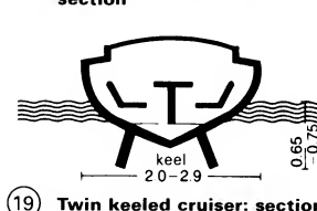
19 Twin keeled cruiser: section
